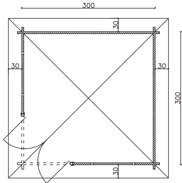
Grundriss / ground plan plattegrund / plan / rzut
